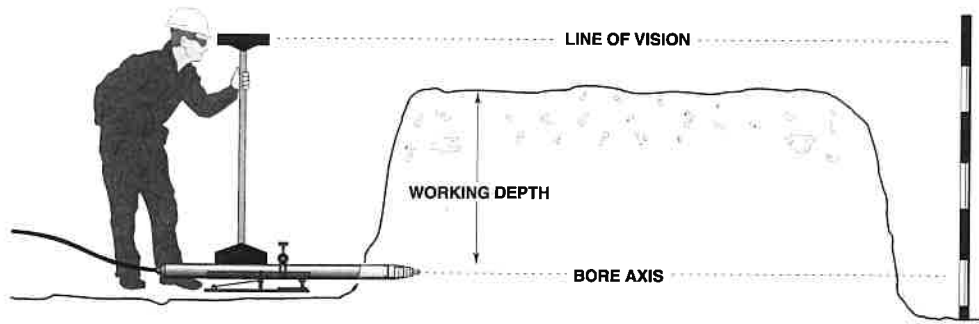
FIG. 6: WORKING DEPTH OF GRUNDOMAT & FIG. 7: ALIGNING THE GRUNDOMAT WITH THE AIMING FRAME.
