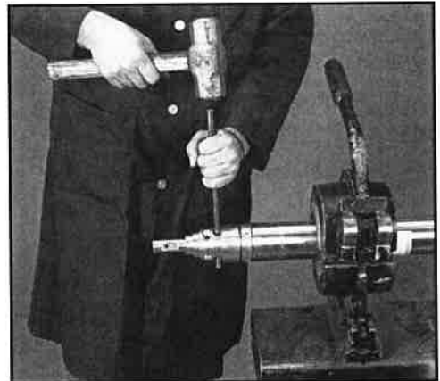
FIG. 20: REMOVING THE ROLL PINS
