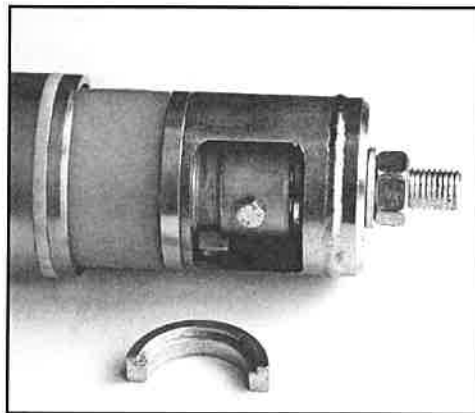
FIG. 67: INSTALLING SEGMENTED RINGS
