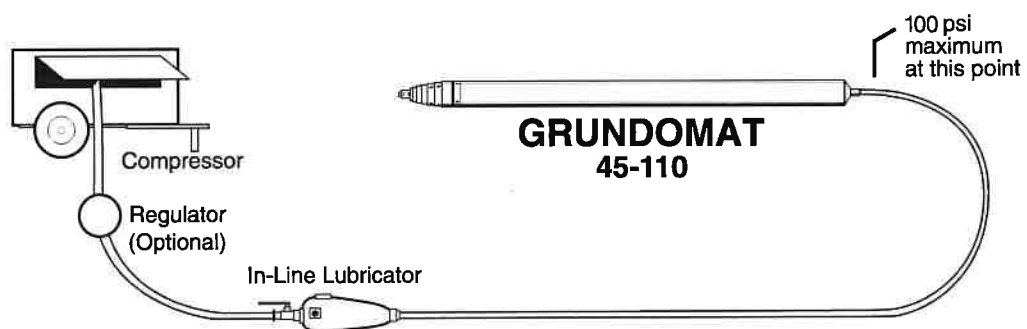
FIG. 2: TYPICAL GRUNDOMAT CONNECTION SEQUENCE MODELS 45-110
