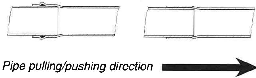
FIG. 13: SLEEVE CONNECTIONS
