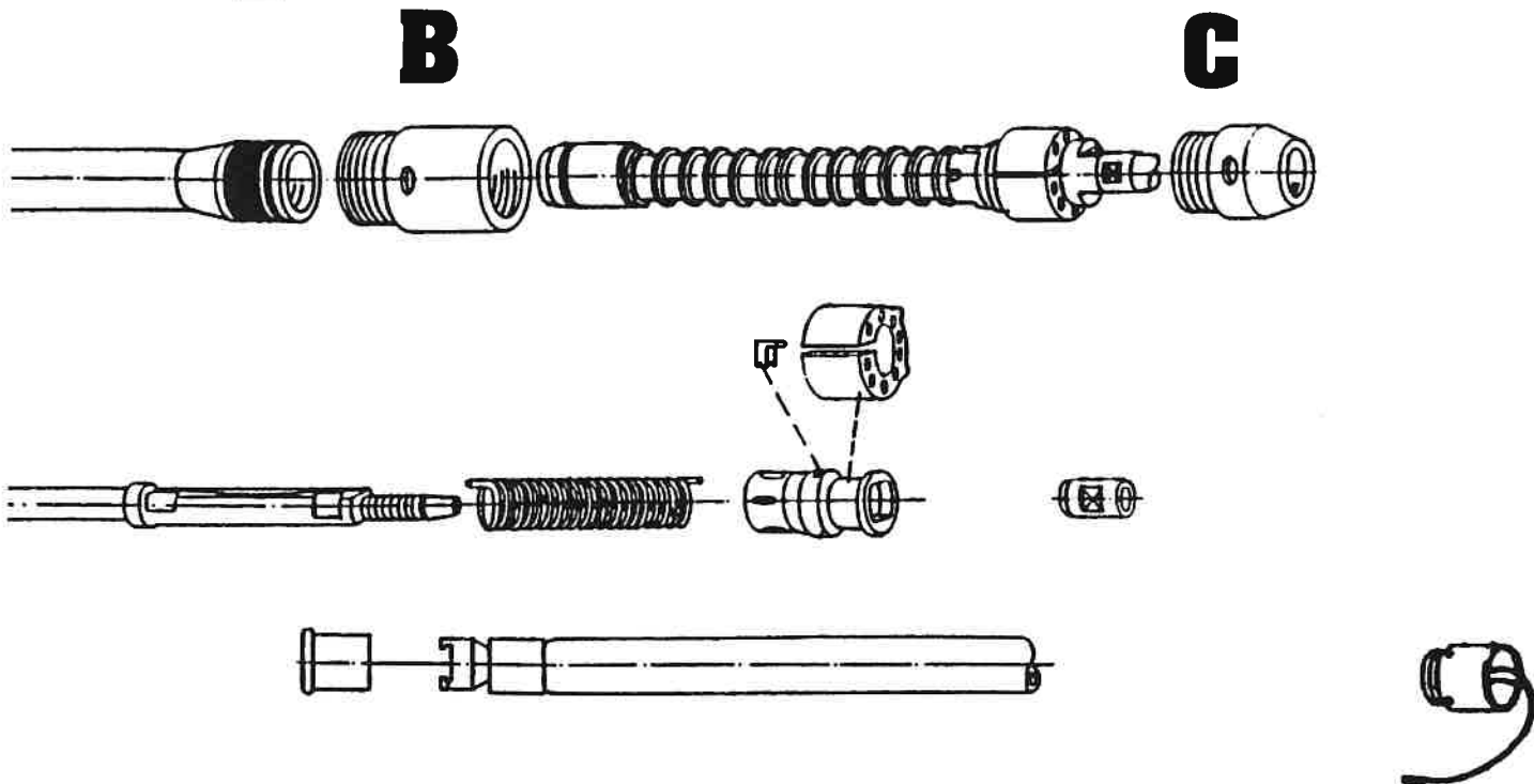
Thread Sealant Usage Chart For GRUNDOMAT*
