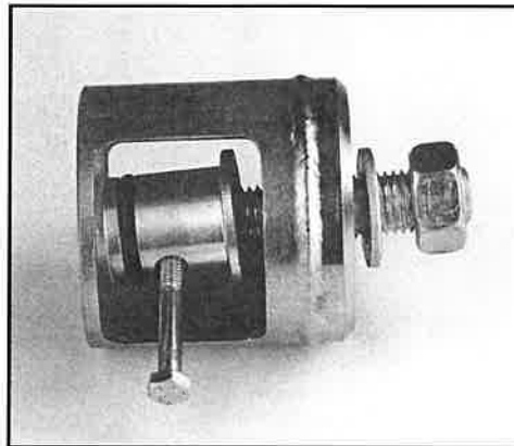
FIG. 60: DISASSEMBLY TOOL
