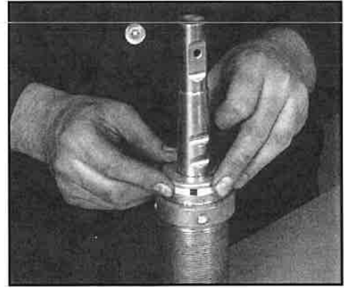
FIG. 29: INSTALL CONE SEAL
