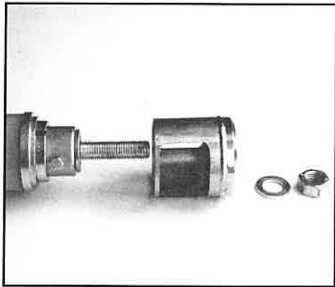
FIG. 66: SECURING BOLT
