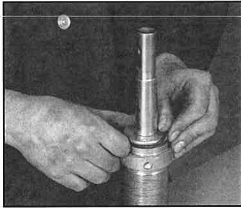
FIG. 28: INSERT O-RINGS
