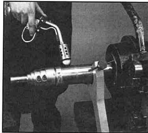
FIG. 17: LIQUEFYING LOCTITE
