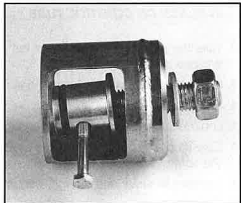
FIG. 65: DISASSEMBLY TOOL
